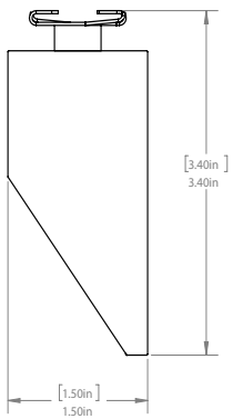
T-Grid 15/16 W/ Drop
