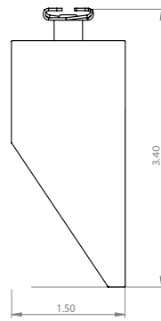
T-Grid 9/16 W/ Drop
