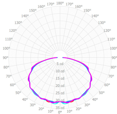
Straight Louver
