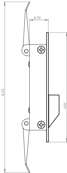
Flange Spring Clip
