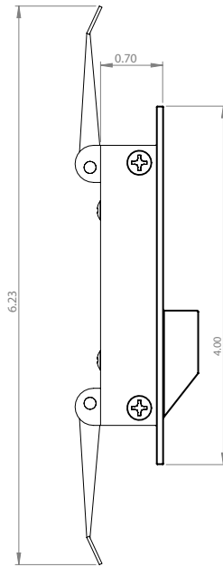
Flange Spring Clip
