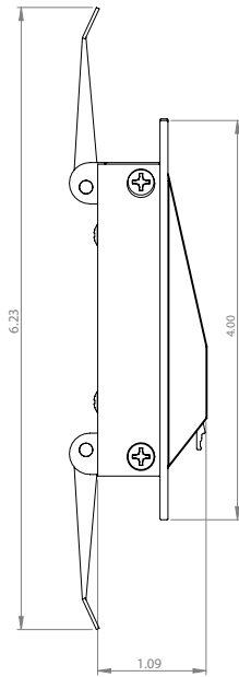
Flange Spring Clip
