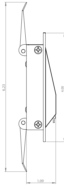
Flange Spring Clip
