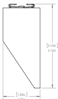
T-Grid 15/16
